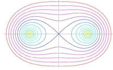
Figure 4: Typical shapes of the Cassini's ovals determined by the equation \mathcal{H}(x_1, x_2) = [(x_1 - 1)^2 + x_2^2] [(x_1 + 1)^2 + x_2^2] = b^4 for b -values ranging from b = 0.1 to 1.5 .
